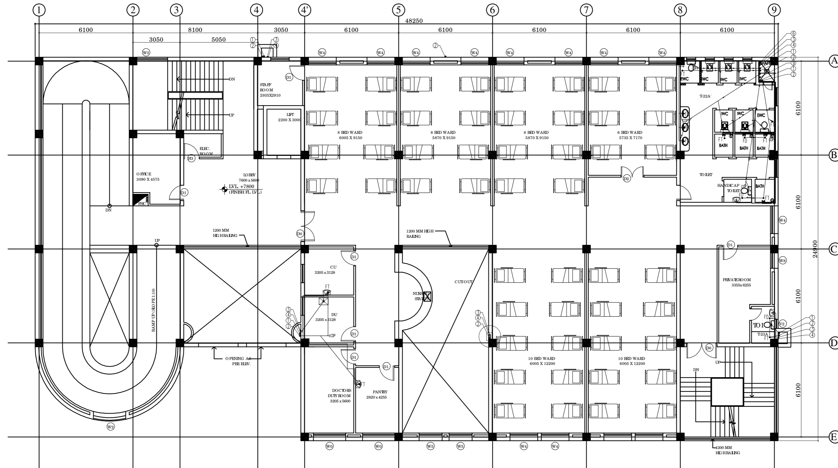
SECOND FLOOR PLAN - 50 BEDS
