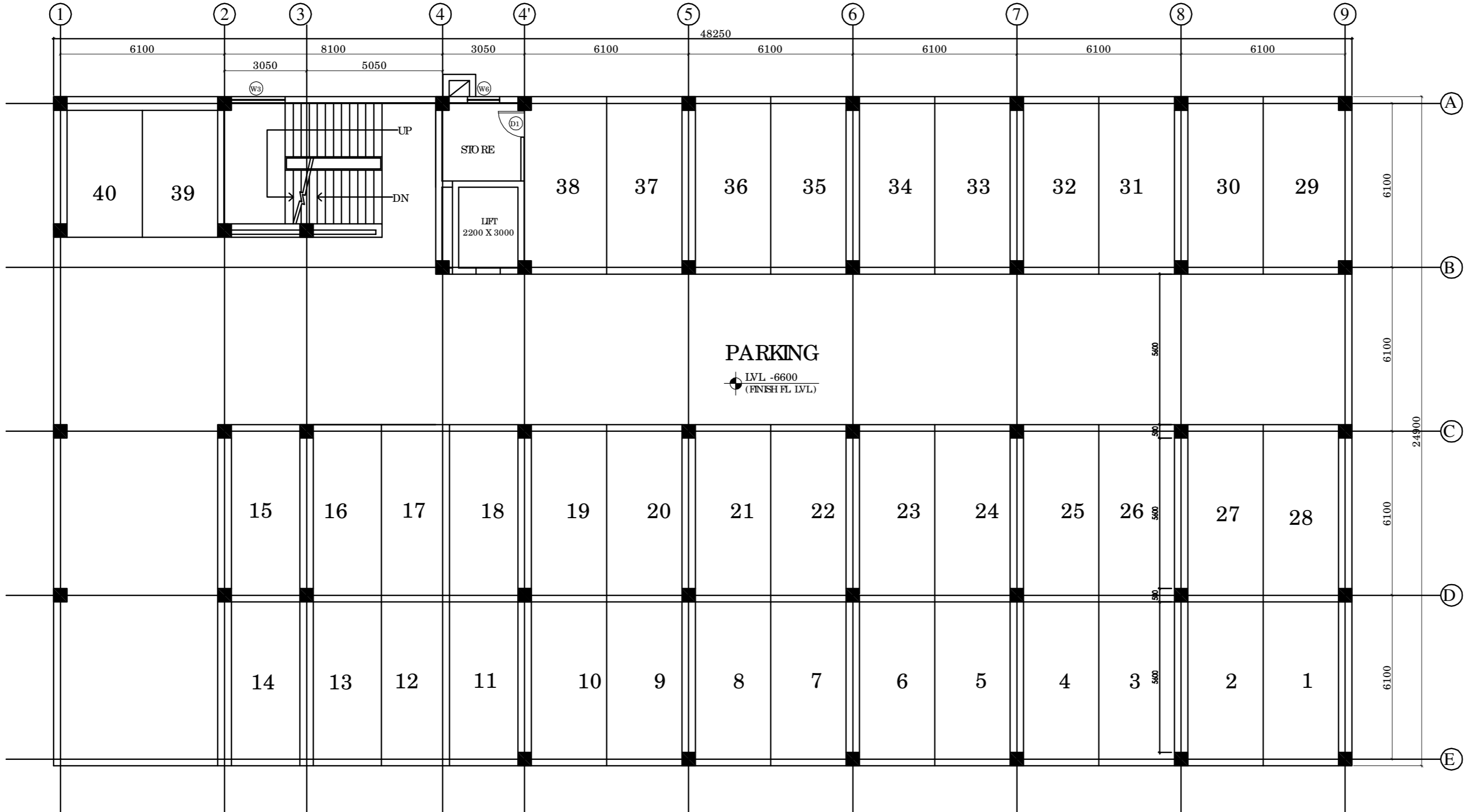
STILT PLAN - 2
