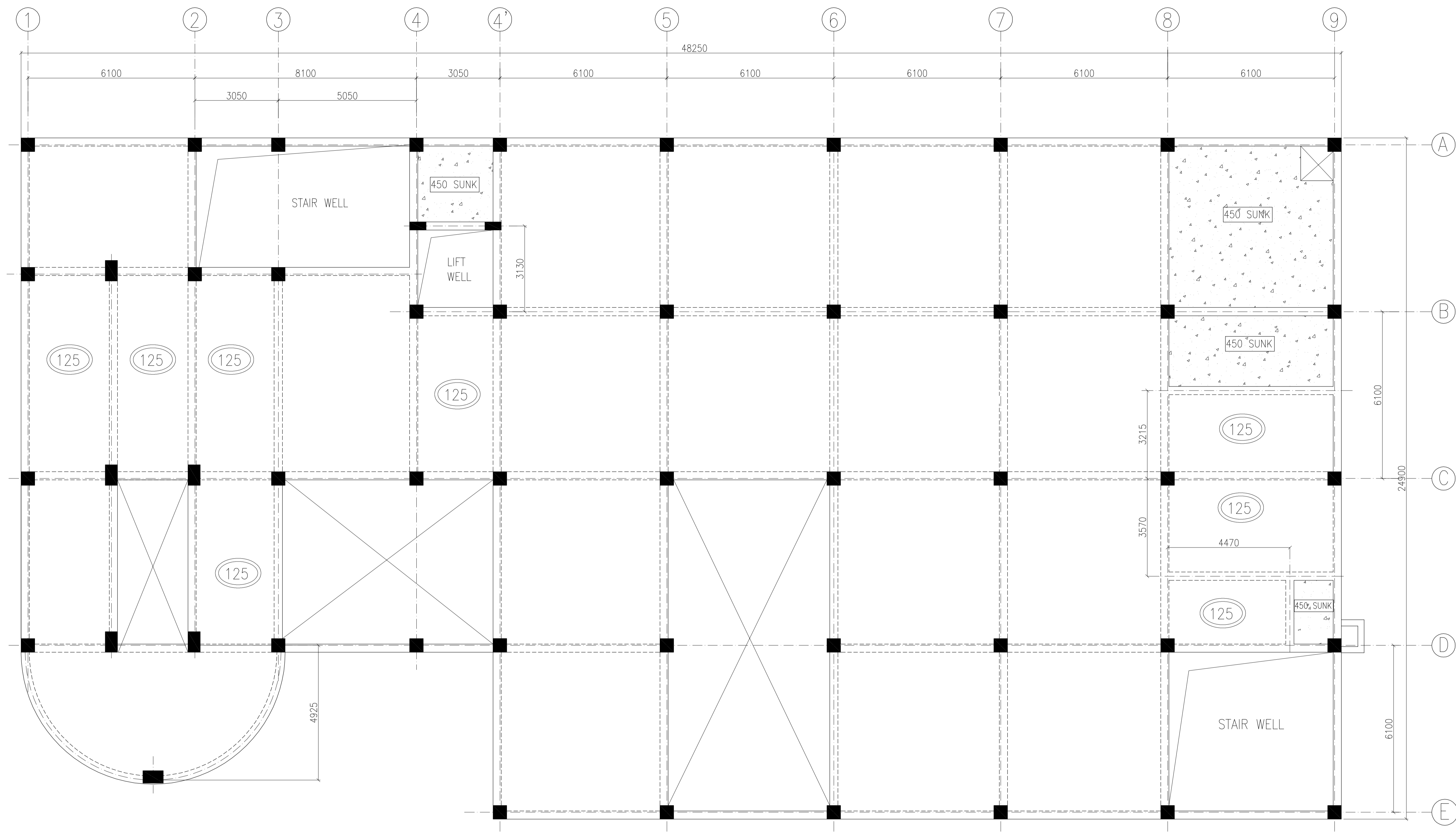
THIRD FLOOR BEAM FARMING PLAN (ALL BEAMS SIZE 300x650 U.N.O.) (ALL SLAB THK. 160MM U.N.O.)
