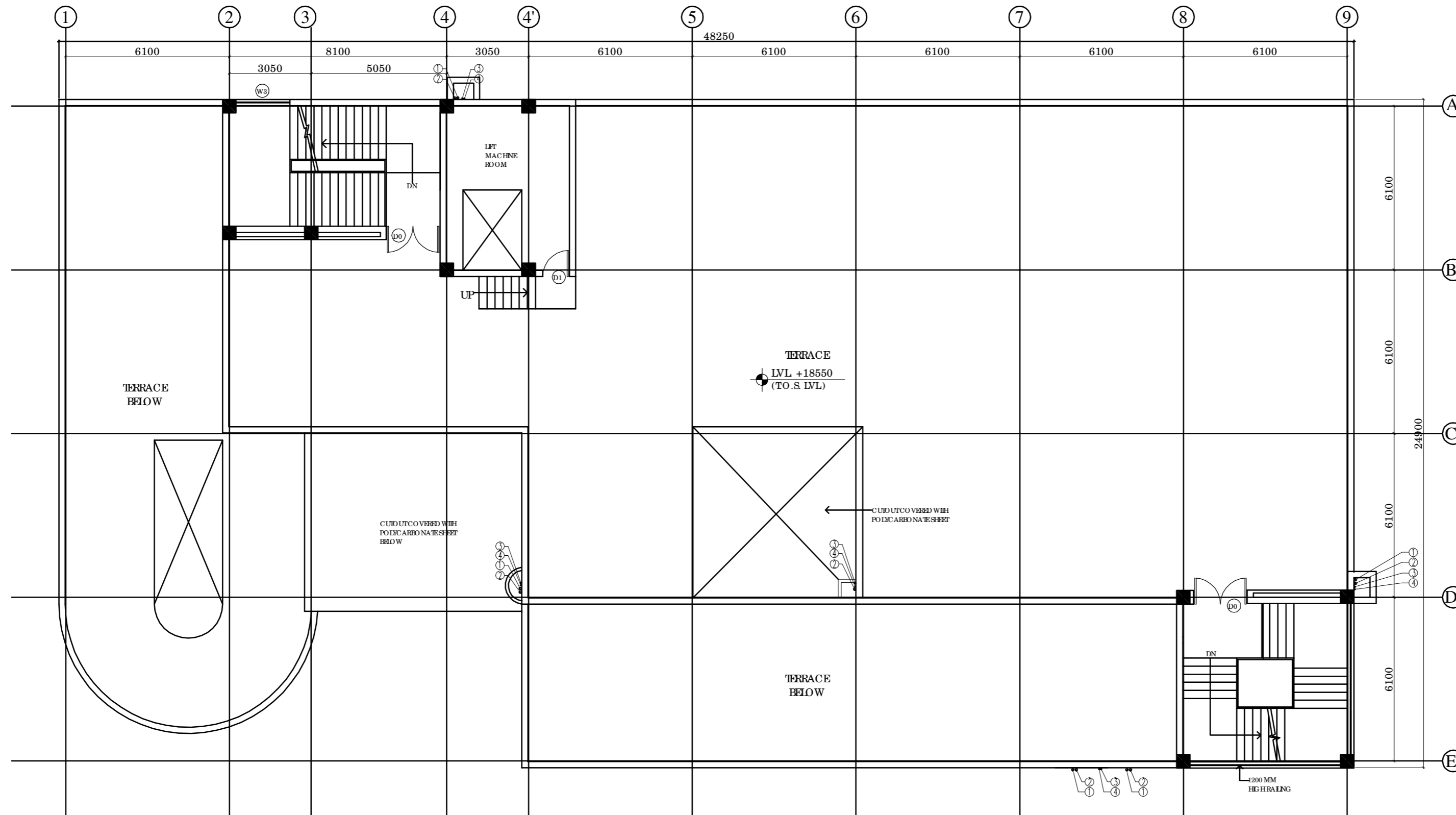
TERRACE PLAN
