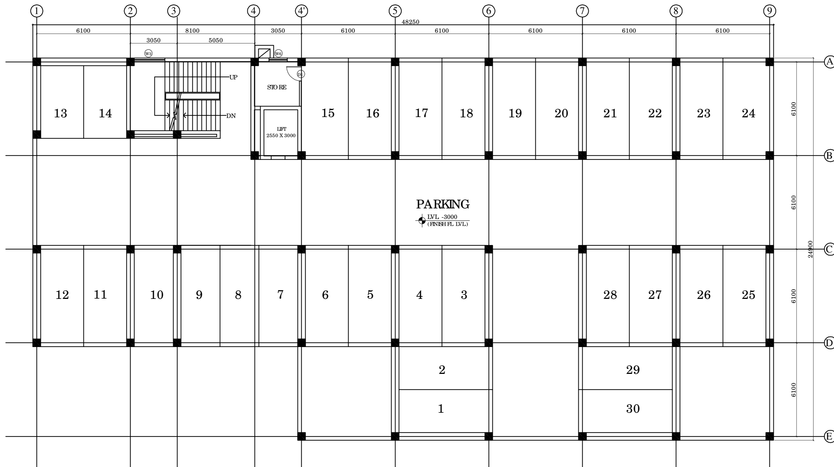
STILT PLAN - 1
